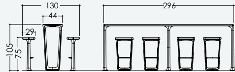
Long Bar Unit 1672 Cast iron and wood 160 kg.
