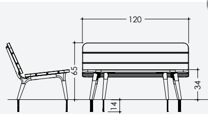
Tzavta picnic Table 1682 Cast iron and wood 124 kg.
