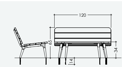
Asif Picnik Table 1686 Cast iron and wood 124 kg.
