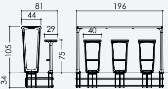
Bar Unit 1670 Cast iron and wood 110 kg.
