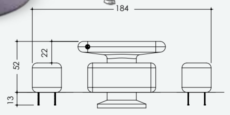
Childrens seating system 1620 Concrete
