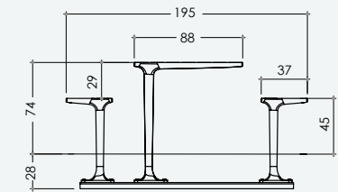
Kerem Picnik Table 1687 Cast iron and wood 180 kg.
