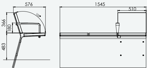
Inbar bench Metal 3 Seats With Armrest 1069 Concrete and metal 250 kg.
