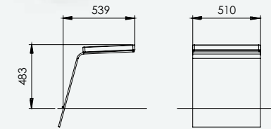
Inbar bench 1081 Concrete and metal 60 kg.
